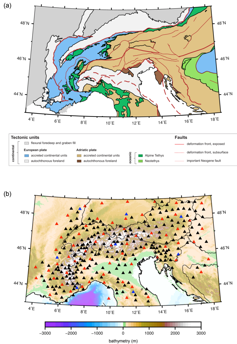
FIGURE 5.1 – Tectonic map and seismic station map of the studied region. (a) Generalized tectonic map of the Alps (Handy et al., 2010), provided by E. Käestle ( http://www.spp-mountainbuilding.de ); (b) Location of seismic stations (triangles) plotted on topographic map. Red triangles : virtual source stations for inversion ; blue triangles : virtual source stations for validation.
