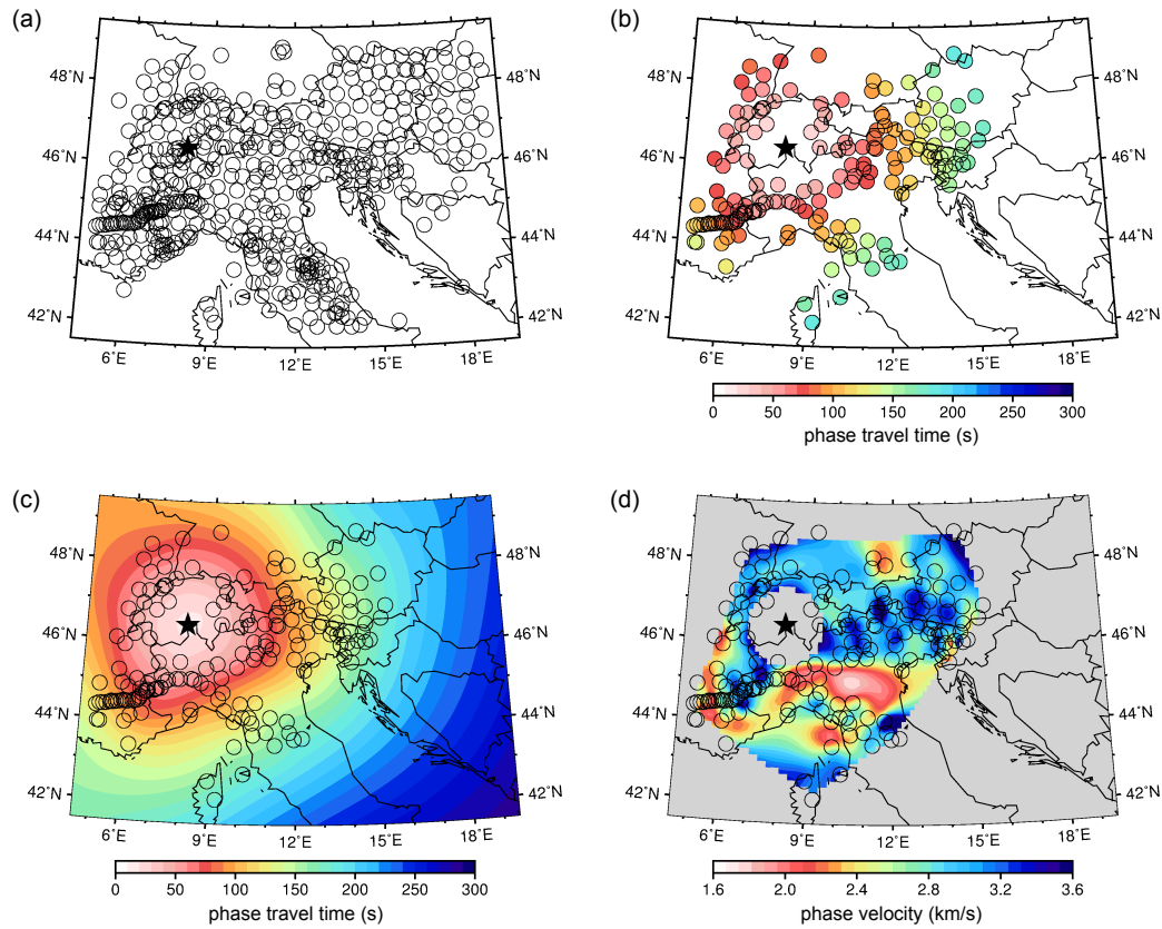
FIGURE 4.4 – Eikonal tomography method, example for a given source station FIESA at 7 s. (a) Location map for the source station FIESA (star) and 482 receiver stations (circles); (b) Available phase travel time measurements of Rayleigh waves between FIESA and receiver stations; (c) Interpolated phase traveltime map; (d) Phase velocities estimated as the inverse of the gradient of phase traveltime map. We discard cells with distances shorter than 4 wavelengths to the source station, as well as areas out of the convex of receiver station distribution. We observe low velocity anomalies in the Po plain and high velocity anomalies in the Alps.
