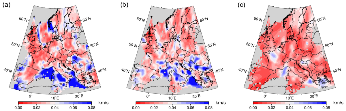
FIGURE 3.17 – Rms errors of inversion results for period bands 5-15 s (a), 15-55 s (b) and 55-150 s (c). We plot only cells with more than 10 crossing paths at 8 s.
